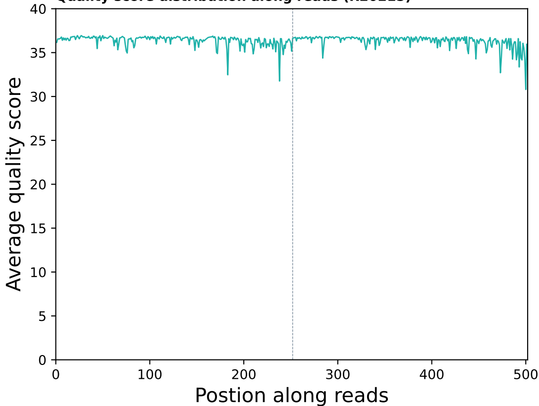
Quality score distribution along reads (R20215)
